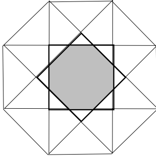
FIGURE 3.2. Flat regular octagon obtained as the union of 16 triangles \triangleleft(\frac{x}{2}, \frac{\pi}{8}) . The shaded interior octagon represents the region with 4 geodesic loops through every point
