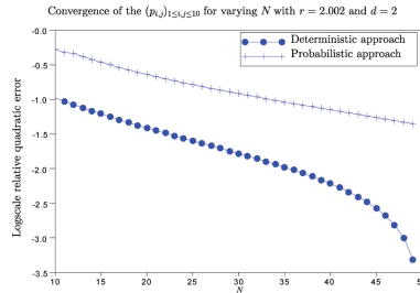
FIG. 4.3. Estimation of the extinction probabilities p_{i,j} when r = 2.002 and d = 2 : Decrease with N of the log of the relative quadratic errors (4.2) between the deterministic and Monte Carlo methods ( M = 200 ).
