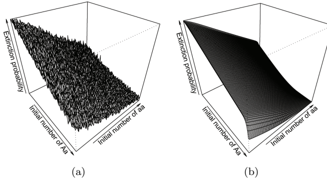
FIG. 4.2. Estimation of the extinction probabilities p_{i,j} when r = 2.002 and d = 2 : (a) with the Monte Carlo method of section 4.1; (b) with the deterministic method of section 4.2.
