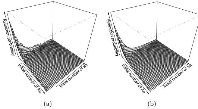
FIG. 4.1. Estimation of the extinction probabilities p_{i,j} when r = 3 and d = 2 : (a) with the Monte Carlo method of section 4.1; (b) with the deterministic method of section 4.2.
