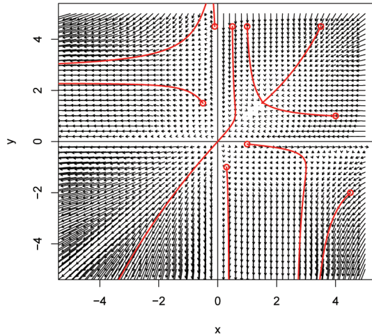
FIG. 3.3. Solutions corresponding to several initial conditions. We see that, depending on the initial condition, the solutions converge or diverge to infinity.
