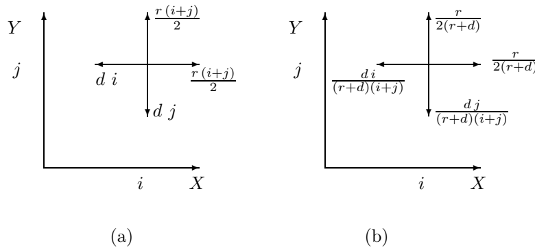
FIG. 1.1. (a) Transition rates for the continuous-time pure-jump Markov process (X_t, Y_t)_{t \in \mathbb{R}_+} . (b) Transition probabilities of the embedded random walk, which we denote by (X_t, Y_t)_{t \in \mathbb{N}} (here and throughout, \mathbb{N} is the set \{0, 1, 2, \dots\} ), with an abuse of notation.
