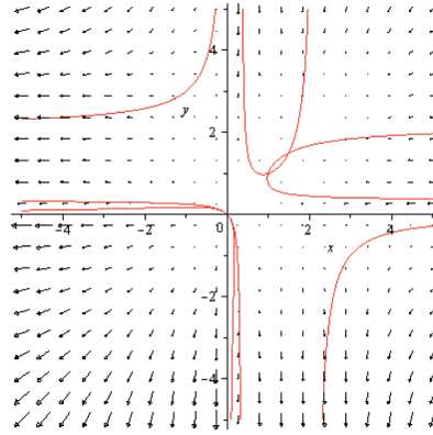
FIG. 3.1. Differential system (3.10): Vector field (Q(x, y), Q(y, x)) . The solid lines correspond to the sets \{Q(x, y) = 0\} or \{Q(y, x) = 0\} .
