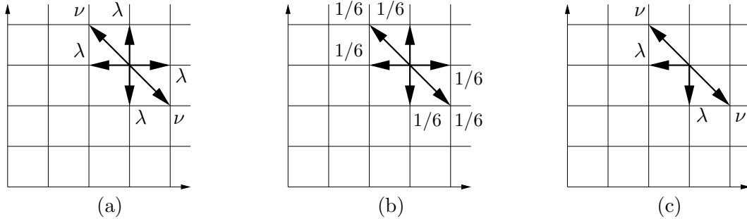
FIGURE 1. Walks considered in [16], [2] and [9], respectively
