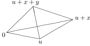
Figure 2: Shift of triangles
