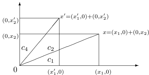
Figure 1: The two descriptions of degree 2 Brownian sheet in \mathbb{R}^2
